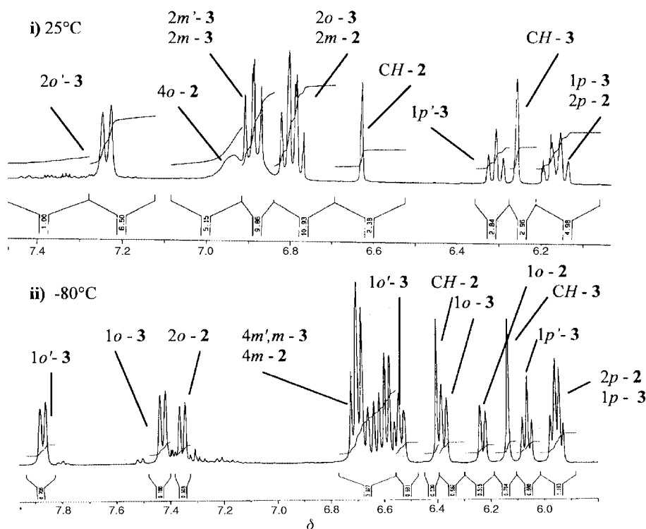
Fig. 2 ^1\text{H} NMR of 2 and 3 in \text{d}_8\text{-thf} . (i) 25^\circ\text{C} , (ii) -80^\circ\text{C} . Note; 3 is unsymmetrical and labelled o , m , p and o' , m' , p' .
