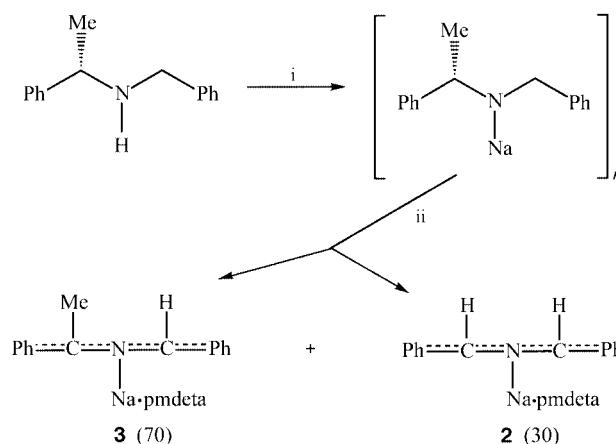
Scheme 1 Transformation of the unsolvated sodium amide to the azaallyl complexes, 2 and 3 . Reaction conditions: i, n BuNa (one equiv.), hexane, 25 °C, 30 min, ii, pmdeta (one equiv.), toluene.
